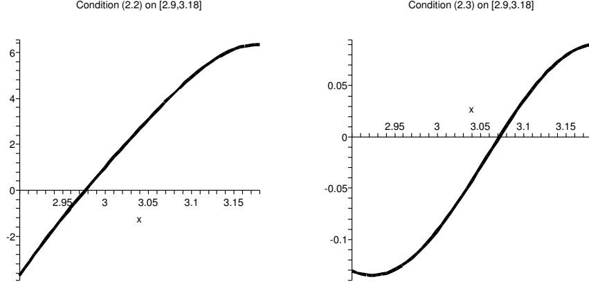
FIG. 2.1. Conditions (2.2) and (2.3) on the interval I_1
