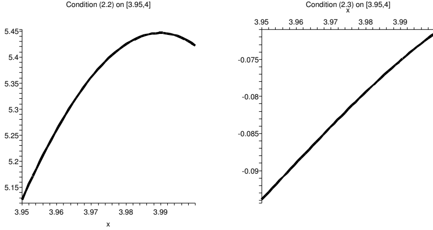
FIG. 2.2. Conditions (2.2) and (2.3) on the interval I_2
