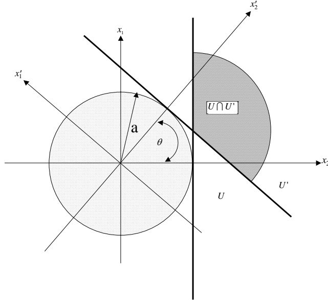
Figure 2: The two functions \phi_{\hat{\mathbf{x}}_2}(\mathbf{x}) and \phi_{\hat{\mathbf{x}}'_2}(\mathbf{x}) are analytic functions in the respective half-spaces U = \{\mathbf{x} : \mathbf{x}_2 > \mathbf{a}\} and U' = \{\mathbf{x} : \mathbf{x}'_2 > \mathbf{a}\} including the common region U \cap U' . The cross-hatched region in the figure depicts a circular subset of the common region.
