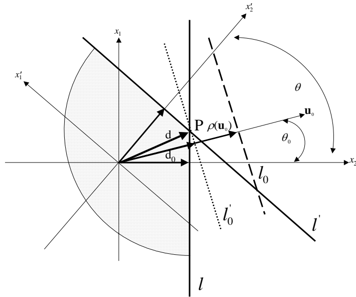
Figure 3: The lines l and l' having unit normals along the directions of the x_2 and x'_2 axes, respectively, intersect at the point labeled P which is at distance d from the origin. A third line l_0 having unit normal \mathbf{u}_0 lying between the x_2 and x'_2 axes at distance \rho(\mathbf{u}_0) from the origin must intersect the two lines l and l' to the left of the point P in order for all three lines to intersect the convex region formed by the intersection of the interiors of the three lines (shown dotted in the figure). The line l'_0 is at the maximum distance \rho(\mathbf{u}_0) for this to occur.
